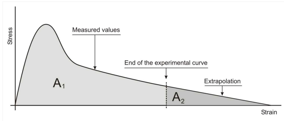
Fig.4: Stress – strain diagram for estimate of fracture energy
