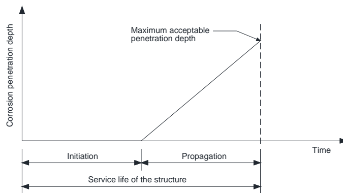
Fig. 2: Tuutti's service life model (after [8]).
